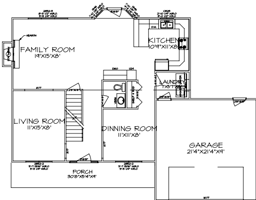
1 FIRST FLOOR PLAN (LOT 308) A-3 SCALE: 1/8"=1'-0" 1/4" SF.
